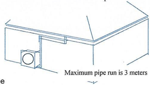
'Back to Back' Installation Example
